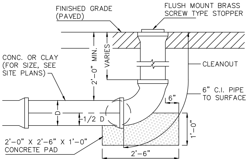
ELEVATION VIEW
