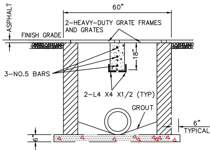
DOUBLE GRATE DETAIL
