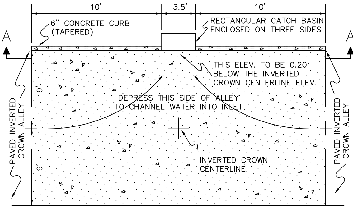
PLAN VIEW
