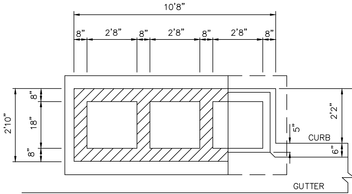
SECTIONAL PLAN (A)
