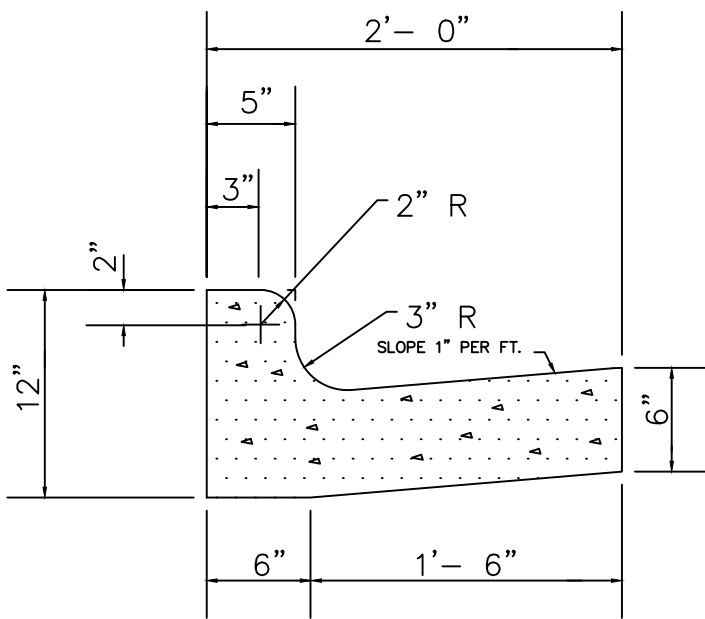
STANDARD TYPE A-24"
