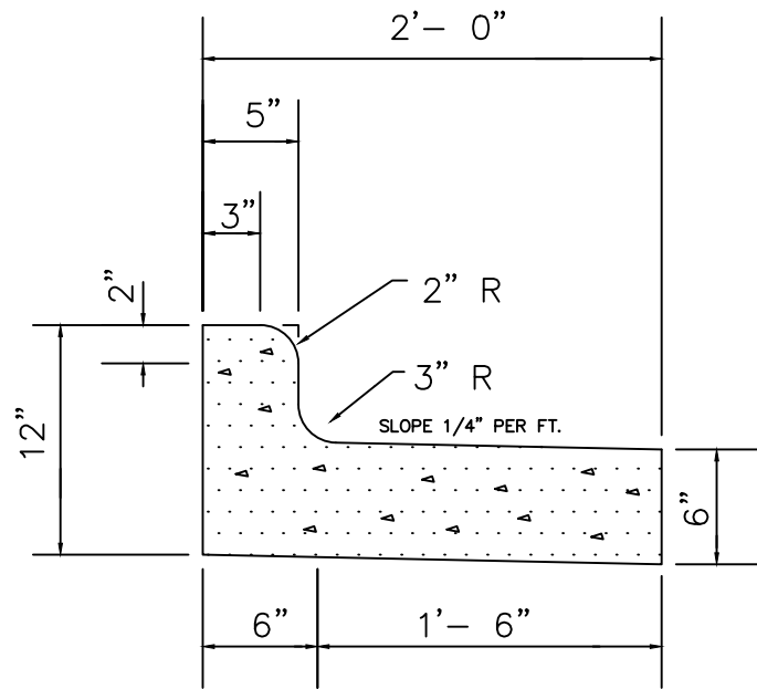
PITCHED TYPE B-24"
